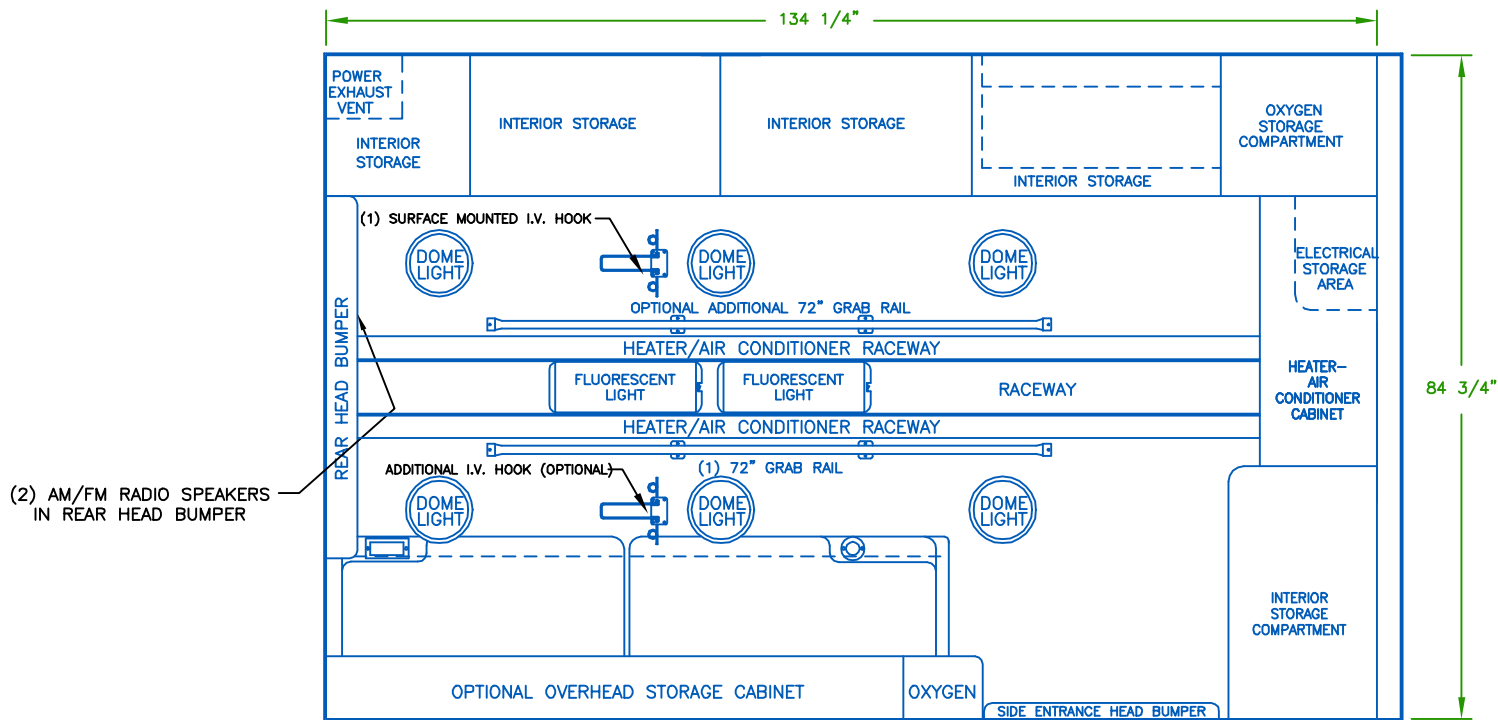
CEILING VIEW
