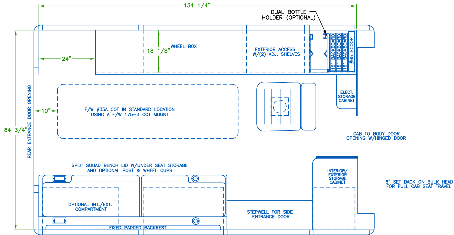
FLOOR PLAN
