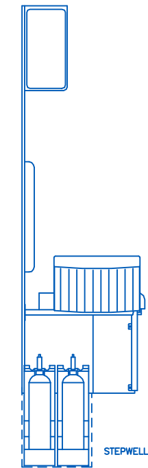
SECTION "A-A" SIDE VIEW
