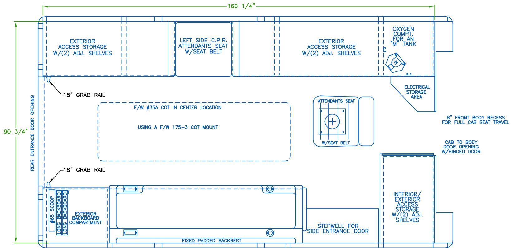
FLOOR PLAN
