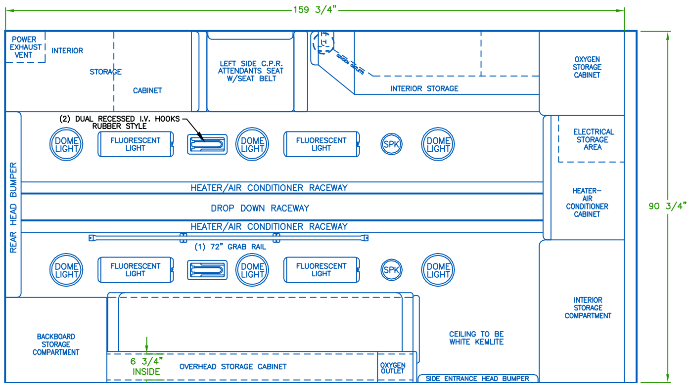
CEILING VIEW
