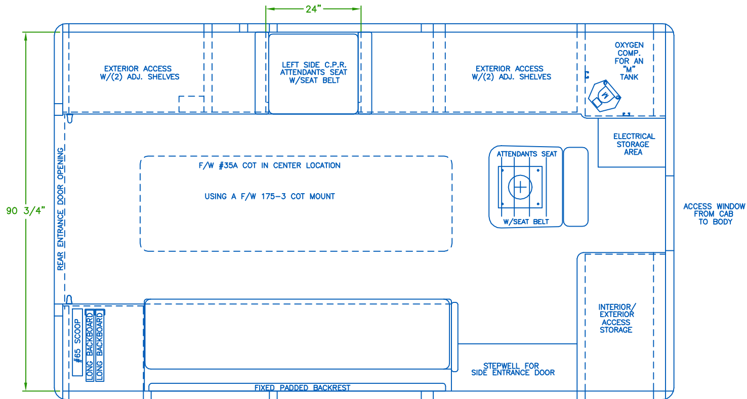
FLOOR PLAN
