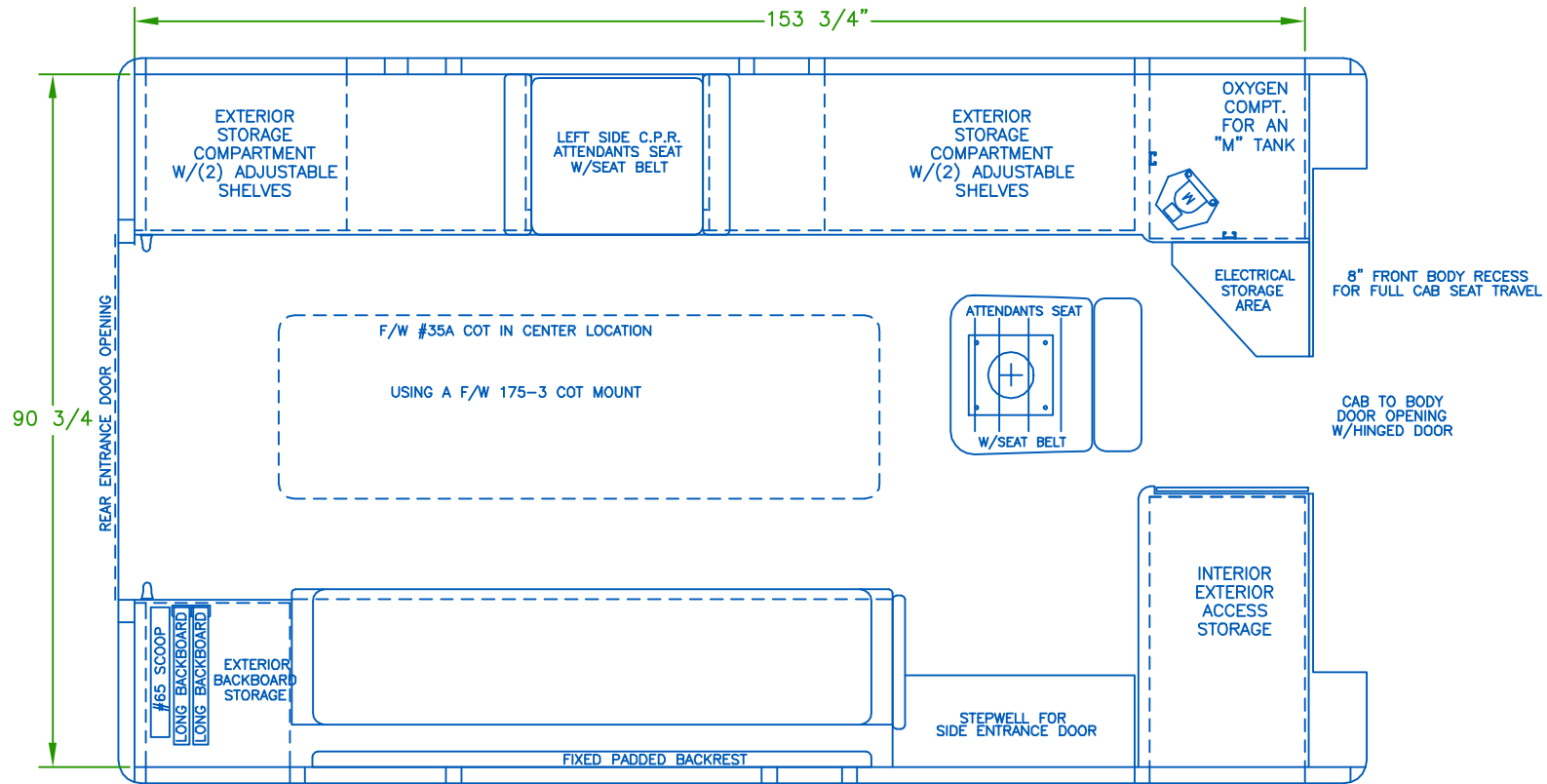
FLOOR PLAN
