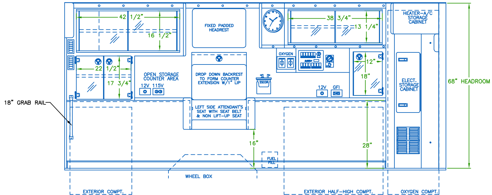
STREETSIDE VIEW
