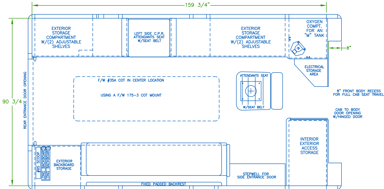
FLOOR PLAN
