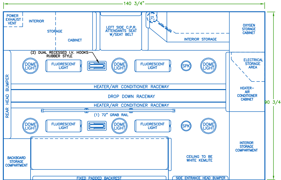
CEILING VIEW
