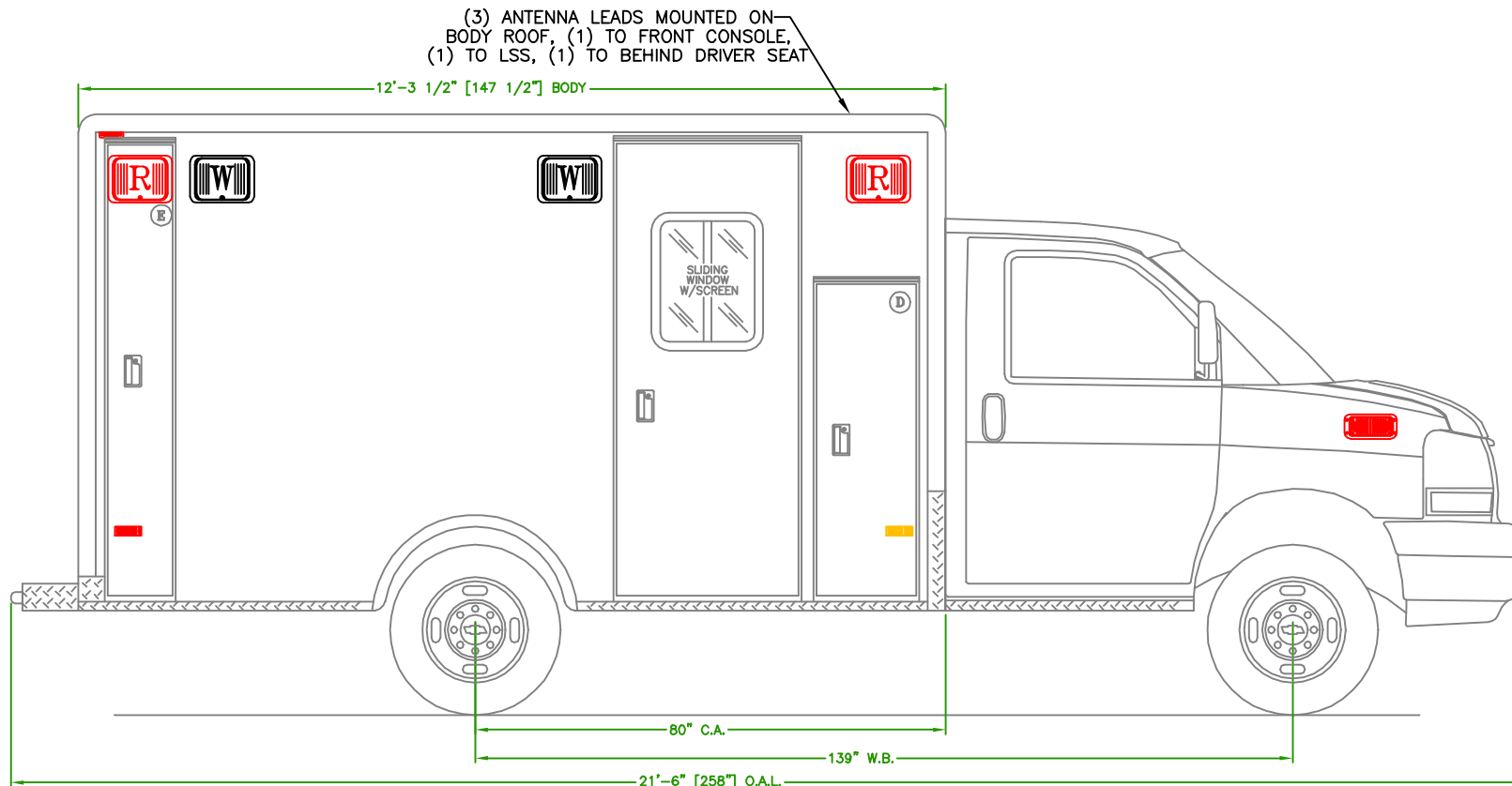
CURBSIDE VIEW
