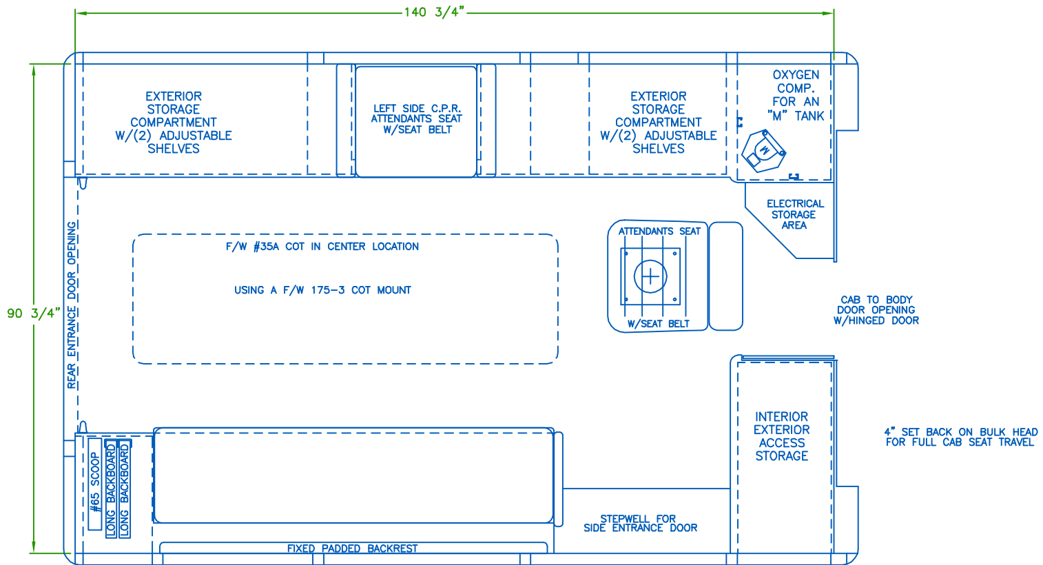
FLOOR PLAN
