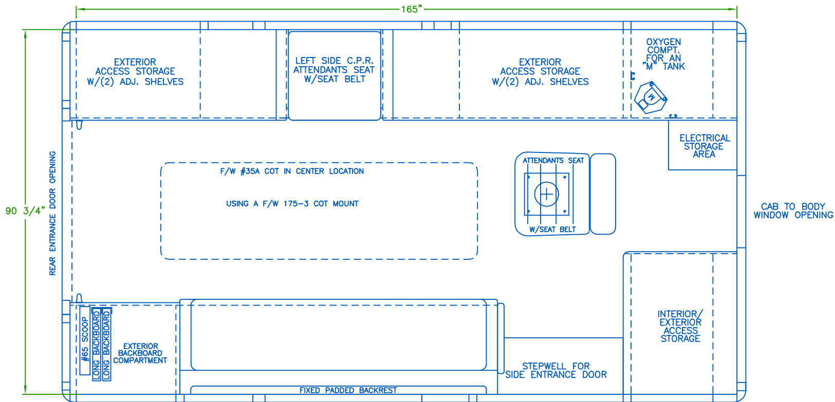
FLOOR PLAN
