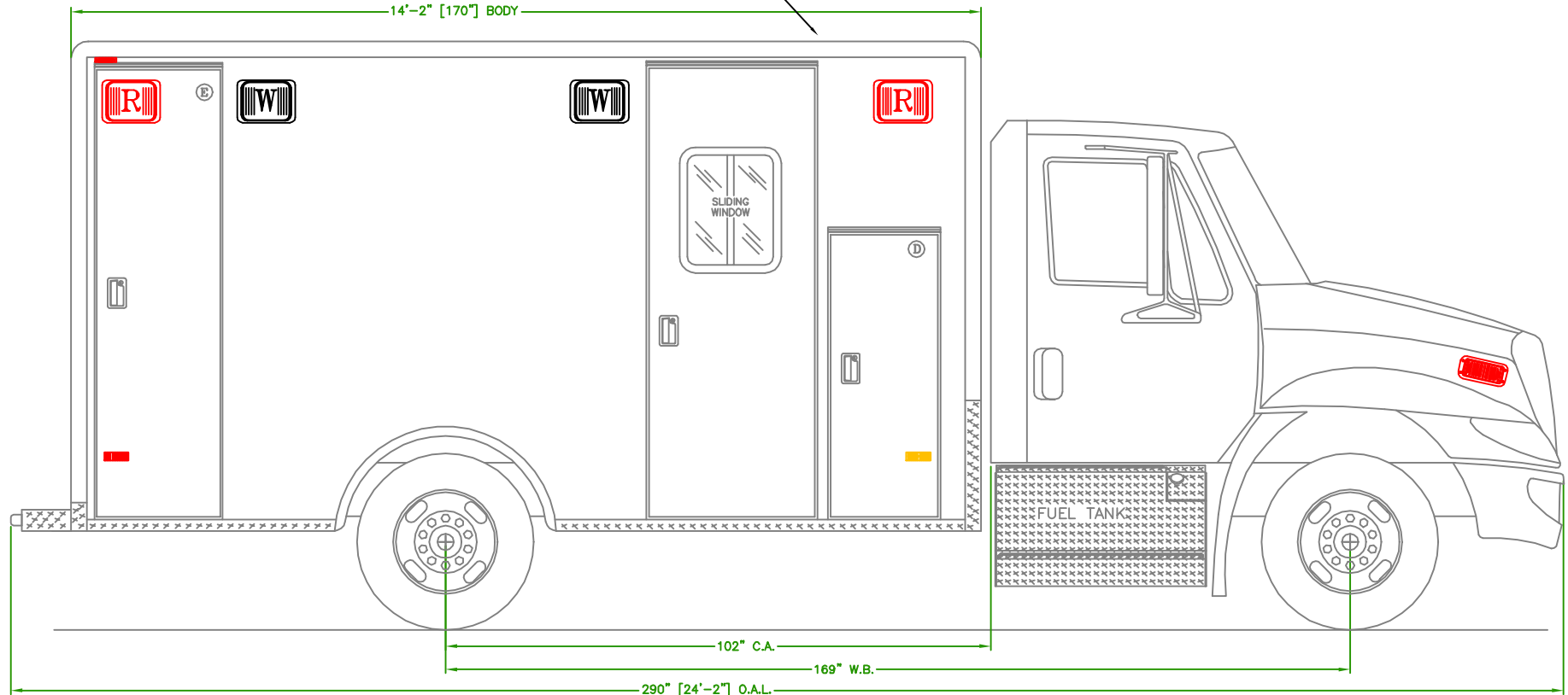
CURBSIDE VIEW
