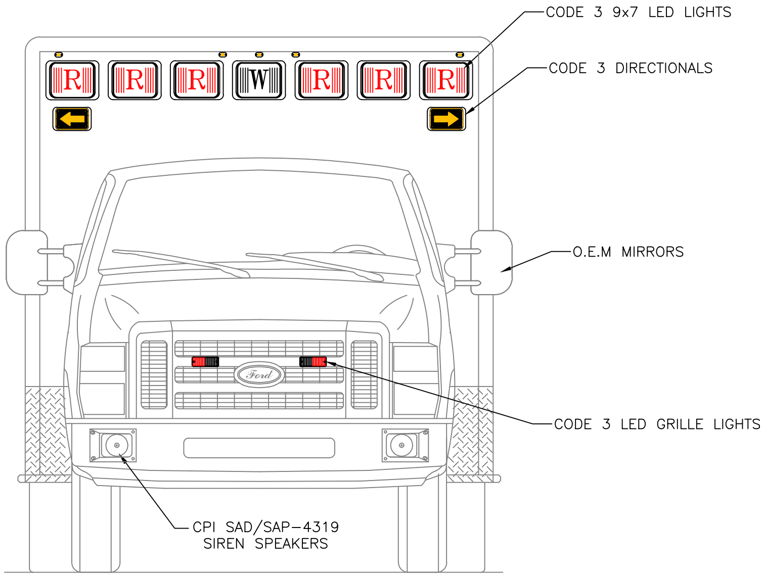
FRONT VIEW
