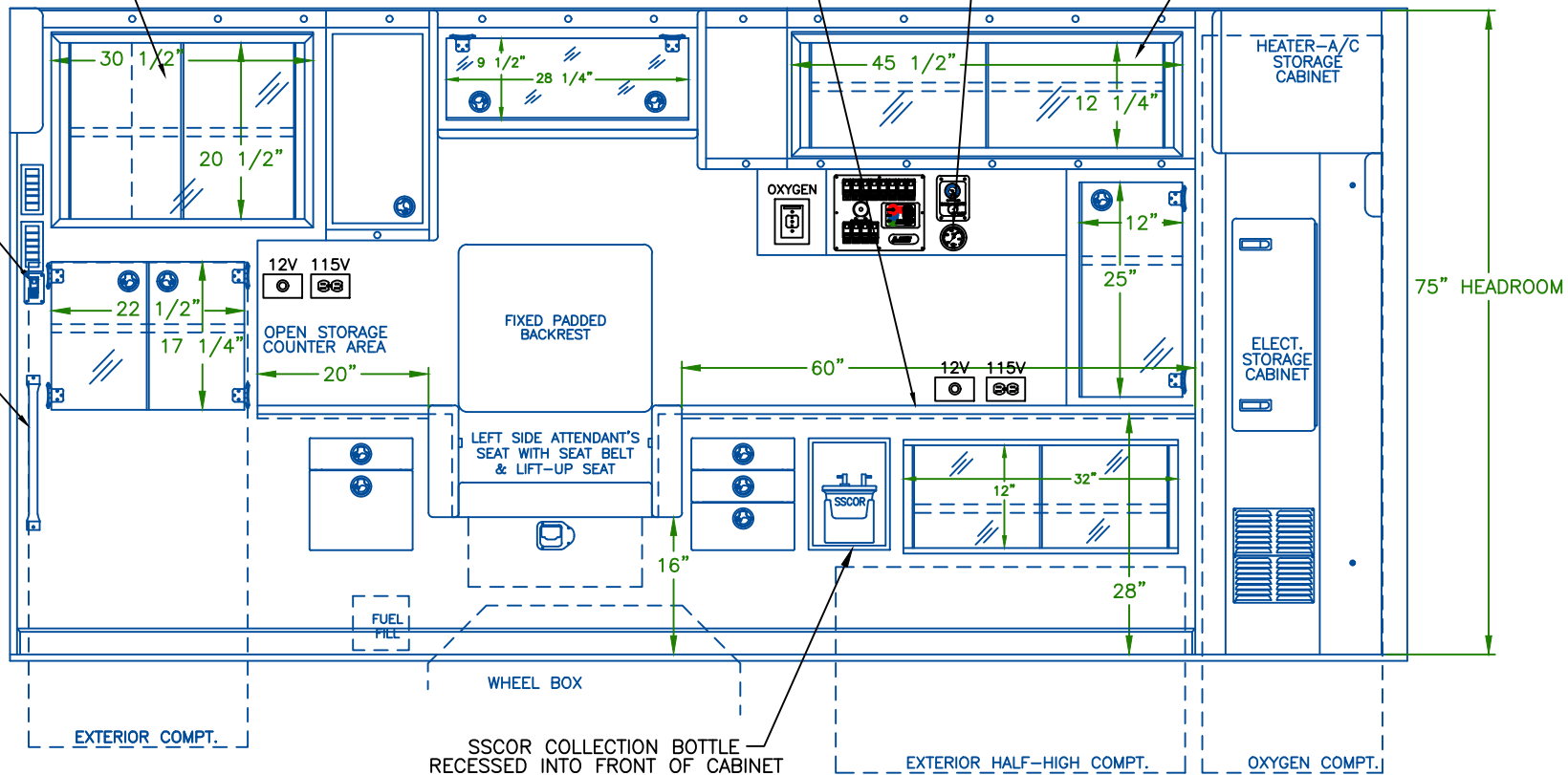
STREETSIDE VIEW
