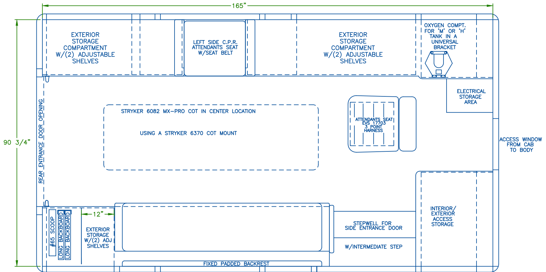
FLOOR PLAN
