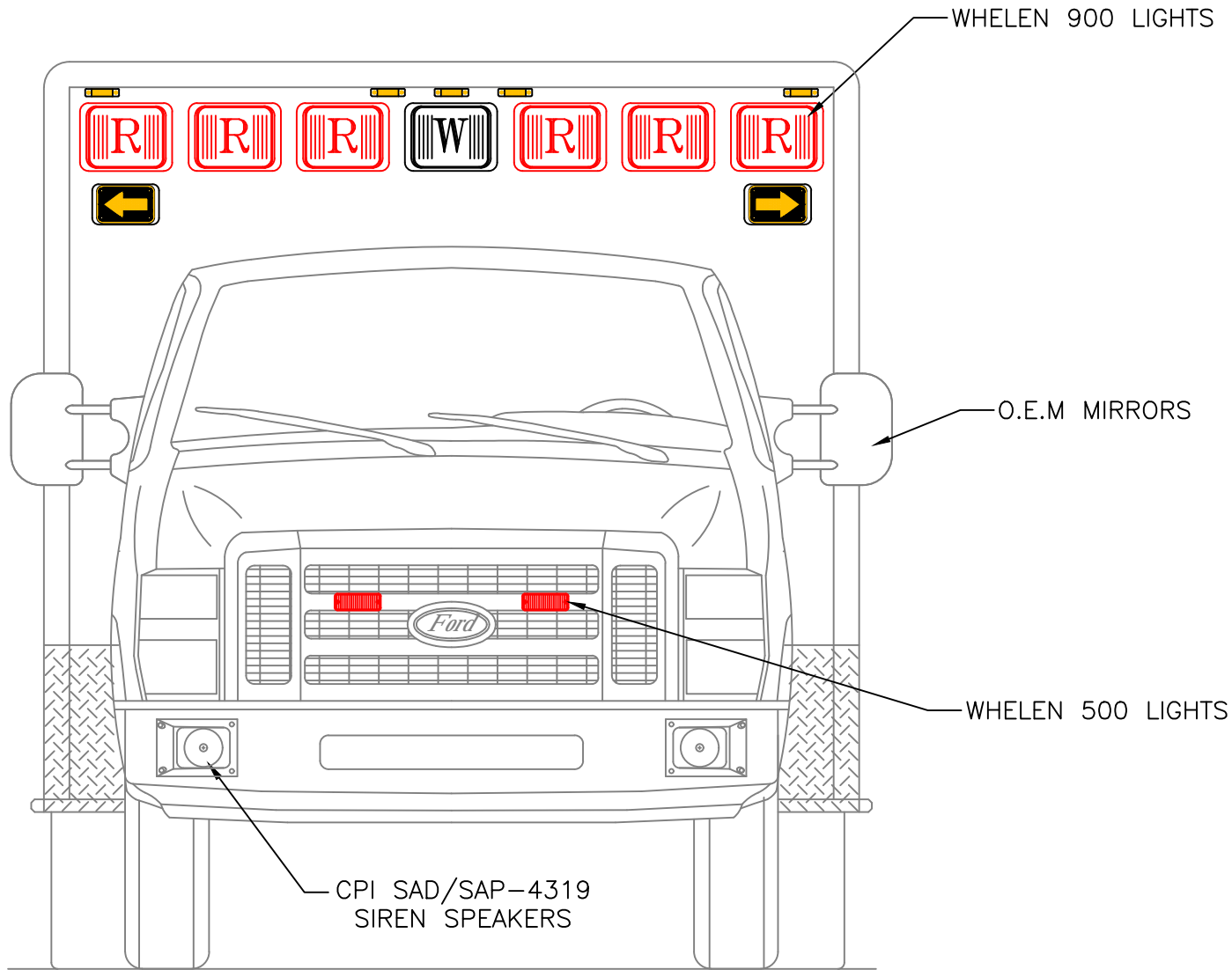
FRONT VIEW
